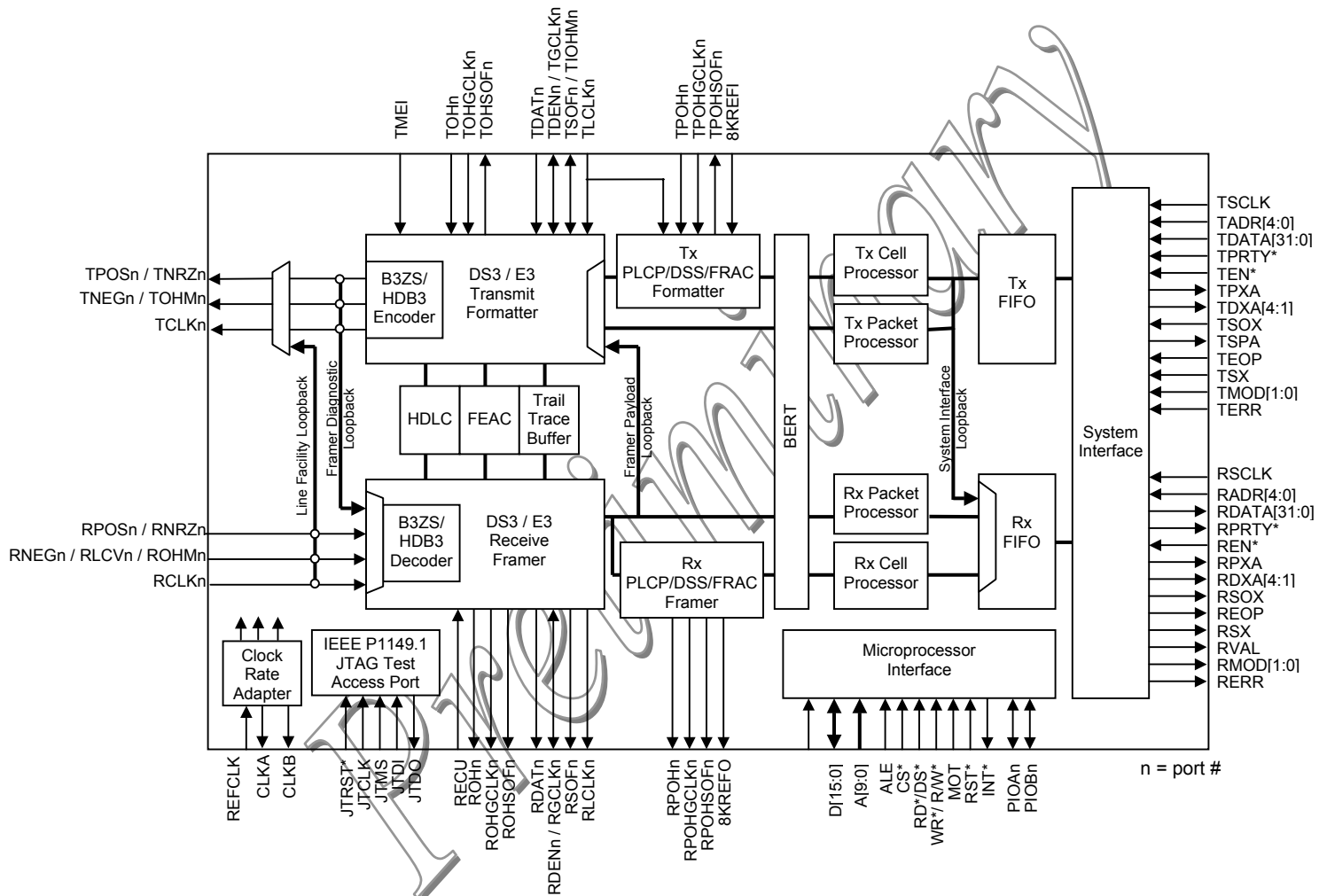
Figure 1–1 Block Diagram
