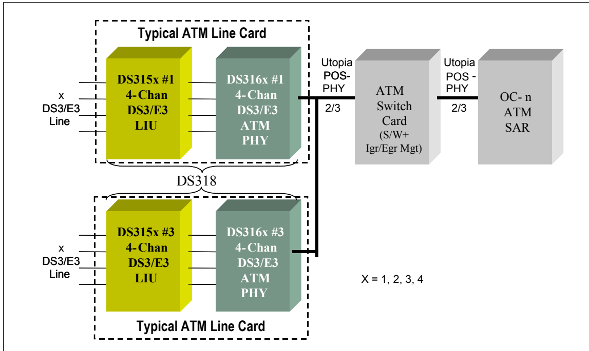
Figure 2-1 Four-Port Unchannelized ATM over T3/E3 Card
