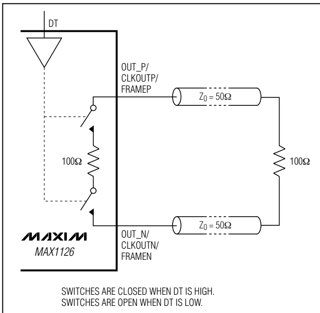
Figure 8. Double Termination
