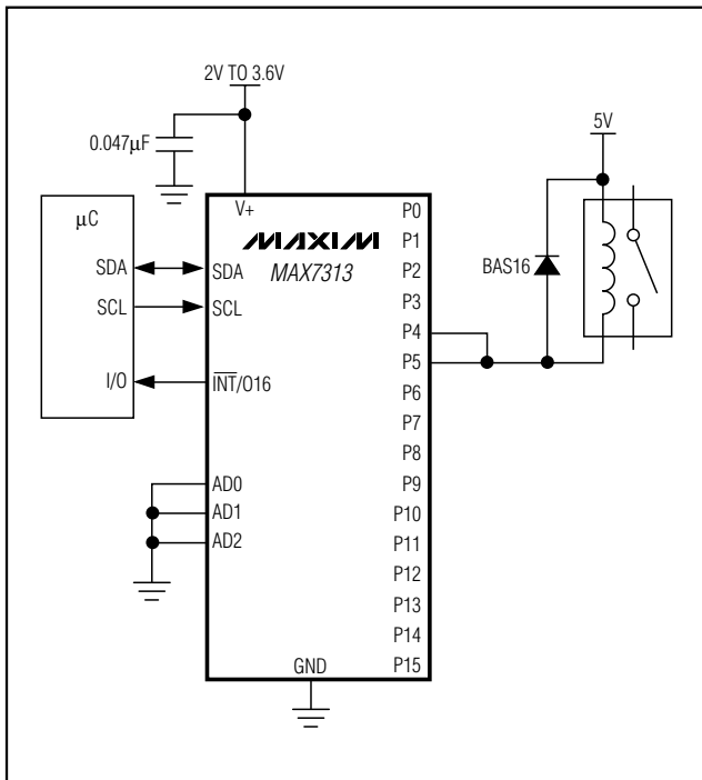
Figure 18. Diode-Protected Switching Inductive Load
